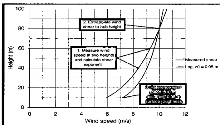
Figure 2 Measured and hypothetical wind shear meeting at 80 m hub height
