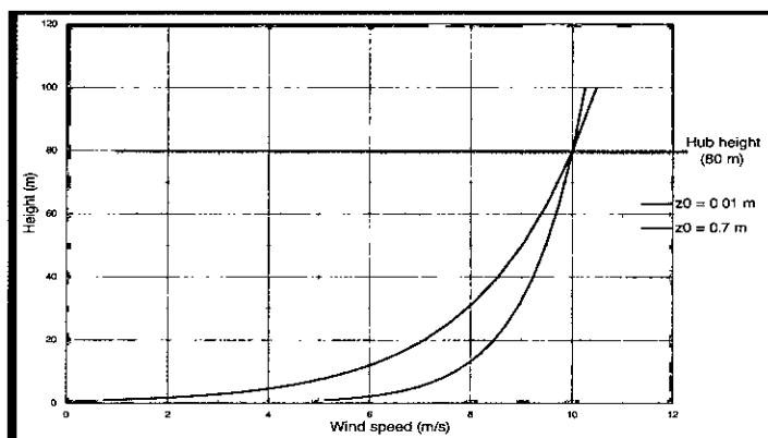
Figure 1 Logarithmic wind shear for two different surface roughnesses (m)
