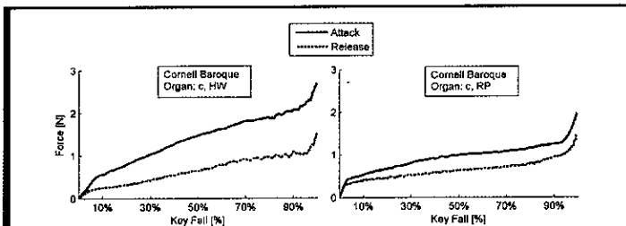
Figure 2 Force at the key tip as a function key fall for tenor c's in Hauptwerk (HW) and Ruck Positiv (RP) for attack and release of the keys. Keys were pressed and released using jolt-free acceleration while the blower was off. The slope of the attack is taken as a measure of the equivalent stiffness in the system, and the area between attack and release is taken as a measure of friction.
