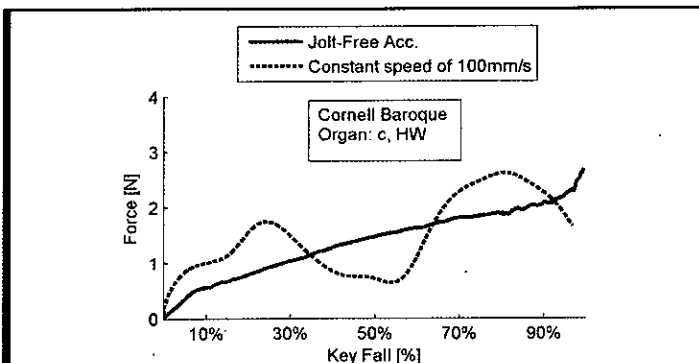
Figure 3 Sample measurement. Force feedback during the attack of the tenor c of Hauptwerk with different playing conditions, while the blower was off. The oscillation during the constant speed condition arises from the inertia of key components.
