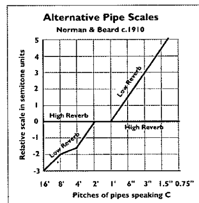
Fig. 10 Norman & Beard pipe scales
