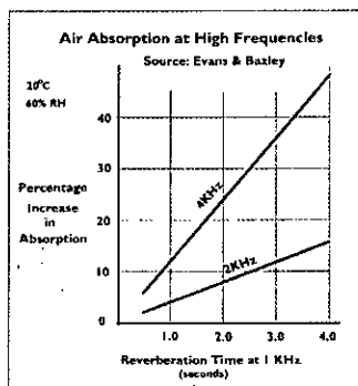
Fig. 8 Air Absorption at High Frequencies
