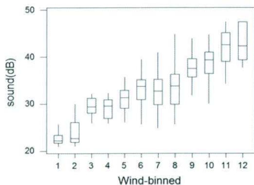
Figure 4: Stacked box plots at each whole number wind speed
