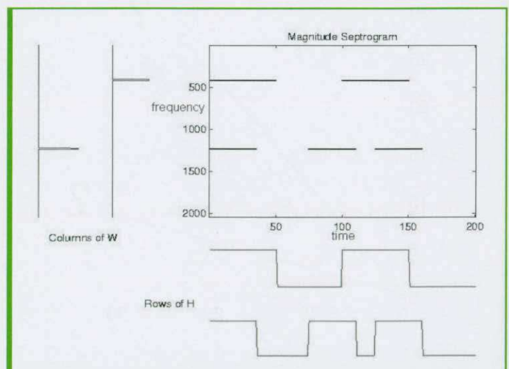
Fig. 8: Illustrative example of decomposition of a spectrogram by non-negative matrix factorization (NMF)
