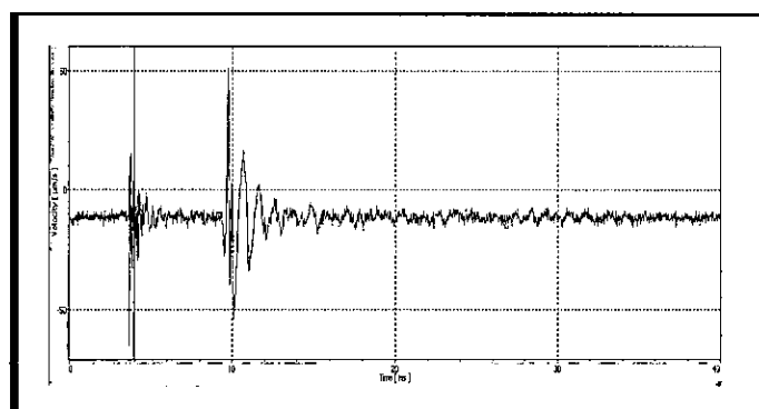
Figure 3 - Measured velocity data for a single point
