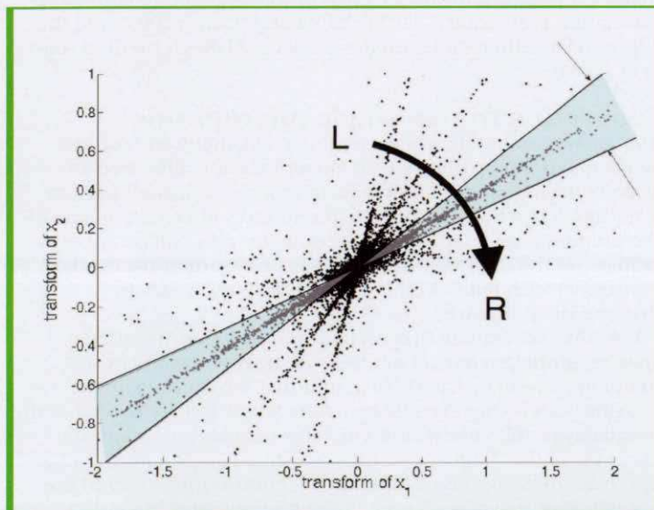
Figure 6: Scatter plot of the real values of a time-frequency transform of panned stereo signal.
