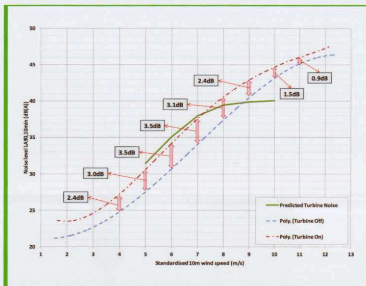
Figure 3 – Variation of noise with wind speed at an intermediate proxy location
