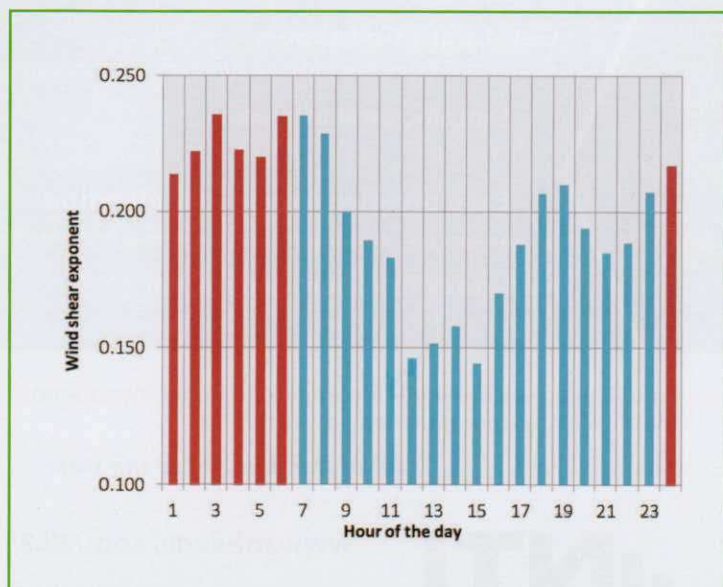
Figure 5 – Typical winter diurnal wind shear variation (with night-time highlighted in red)
