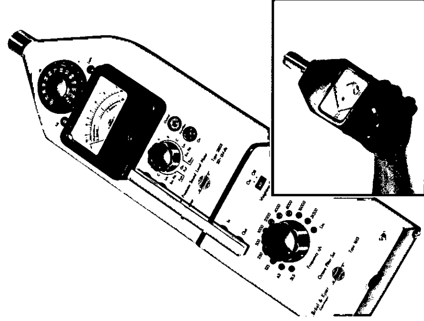
Figure 1 Contrasting sound level Meters of the 1960s. At the top, the B&K 2203 the first meter to the International Standard and below Acos SLM 3 with limited functionality but to the same standard and cost only 10% of the B&K unit. Today B&K still exist and Acos do not.
