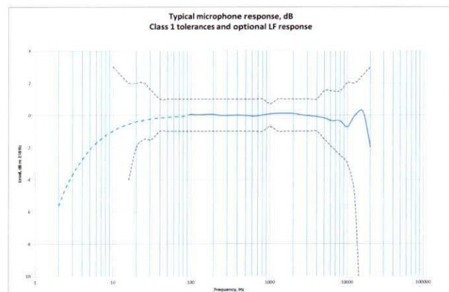
Figure 5 Typical microphone response, with optional LF extension
