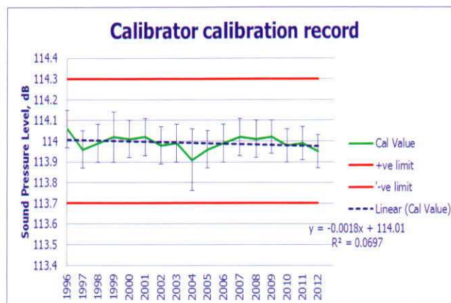
Figure 10 Calibrator periodic verification record for drift analysis
