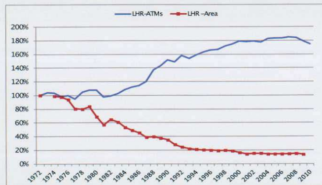
Figure 5 - Normalised Area within 57 dBA 16-hr Leq/35 NNI contour and ATMs for Heathrow. (1972 = 100%. No Area data for 1973 or 2010.)
