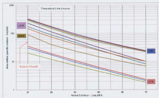
FIGURE 6 - Relationship between contour area and noise level for 1988, 1989 and 1990 for Heathrow (LHR), Gatwick (LGW), and Stansted (STN), and for Manchester (MAN) for 1990. Also shown is the relationship for a theoretical line source and for the 'Rule-of-Thumb'
