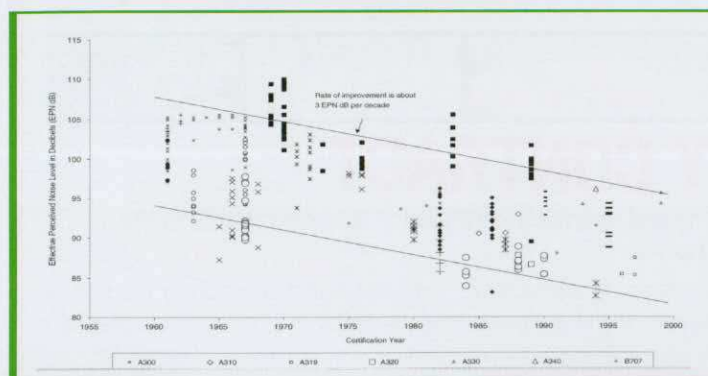
Figure 2 - Trend in reduction of aircraft 1955 – 2000 and EPNdB ratings of A300 types
