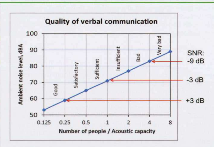
Figure 3. The relation between ambient noise level and number of people relative to the acoustic capacity. Also shown are the regions of different quality of verbal communication.
