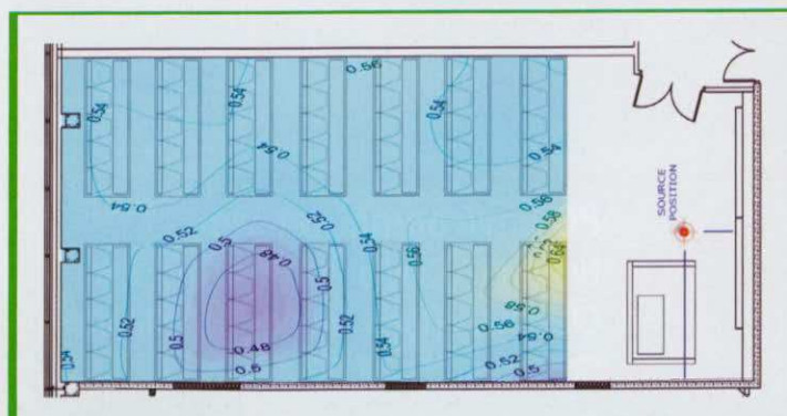
Figure 3 – Room STI map for Room 5, the 'worst' performing room according to STI
