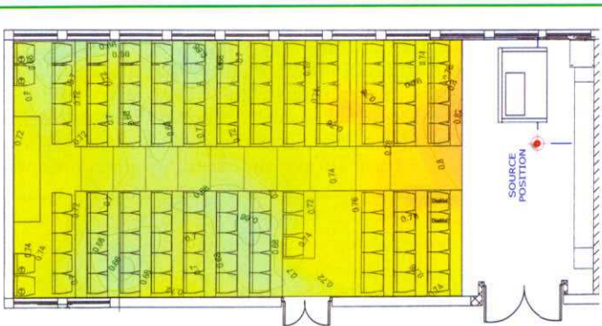
Figure 4 Room STI map for Room 3, the 'best' performing room according to STI
