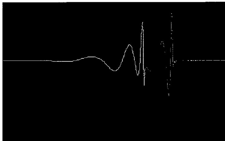
Figure 2: The travelling wave generated by two quiet tones of different frequencies in a healthy cochlea. The waves reach distinct large peaks with the lower frequency travelling further than the higher frequency.
