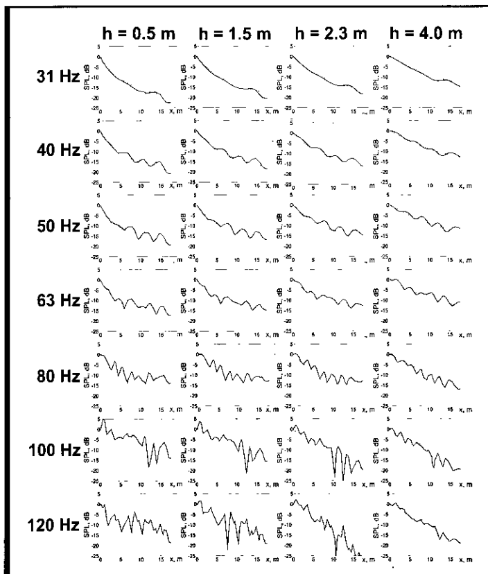
Fig. 6 Sound pressure level distribution over distance at different heights and different frequencies with and without the audience. Solid line represents results with the audience present, dashed line – without audience.
