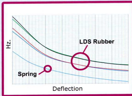
LDS / Spring Dynamic Stiffness Curves
