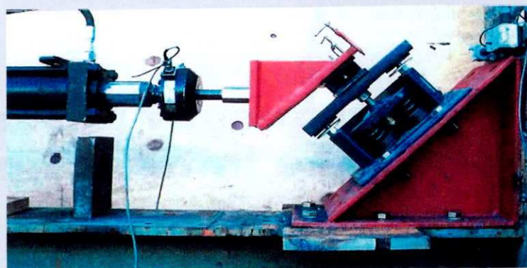
Spring Mount testing
