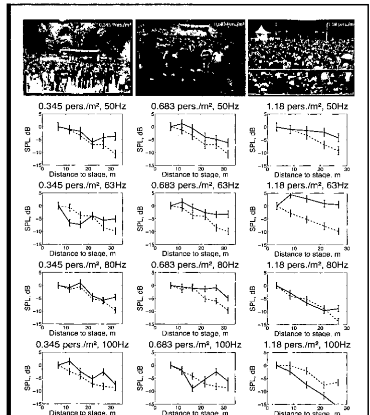
Fig. 8 Live measurements results. Solid line – filled venue, dashed line – empty venue, dotted line – ideal point source.
