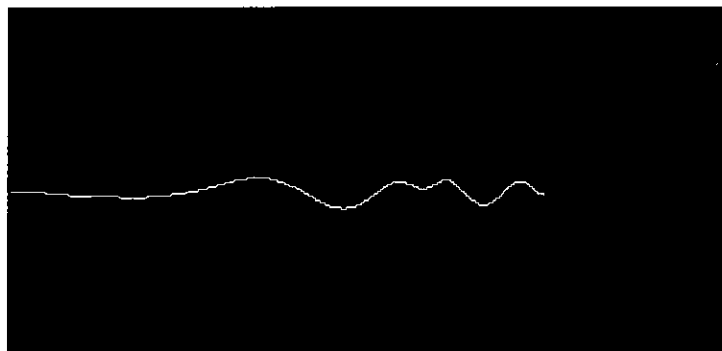
Figure 3: The travelling wave generated by two quiet tones in a cochlea with damaged OHCs. The peaks of the two tones are smaller and are indistinct. These changes in the shape of the travelling wave reflect typical patterns of hearing loss. Frequency discrimination is worse because the peak of the wave is broader and quiet sounds are lost because the peak is smaller. The travelling wave for loud sounds (as studied by Von Bekesy) is relatively unaffected by OHC loss.
