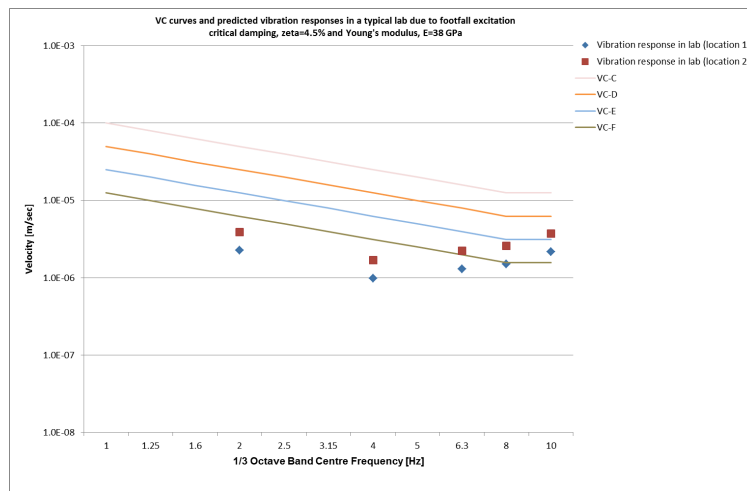
Figure 2: vibration response in a typical lab due to footfall excitation. Material properties of concrete: critical damping, \zeta=4.5\% and Young's modulus E=38 GPa
