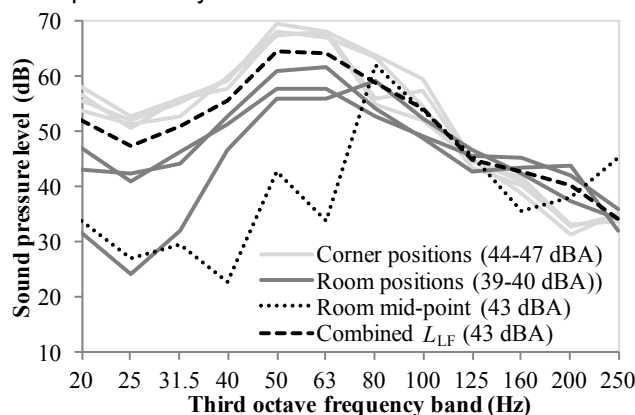
Figure 7: spatial variation in structure-borne noise levels in a small room
