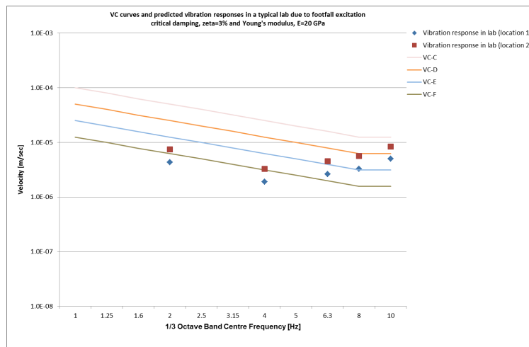
Figure 3: vibration response in a typical lab due to footfall excitation. Material properties of concrete: critical damping, \zeta=3\% and Young's modulus E=20 GPa
