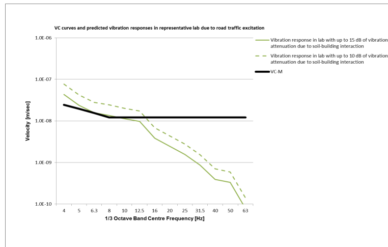
Figure 5: vibration response in a typical lab due to road traffic excitation with different soil-structure coupling loss factors
