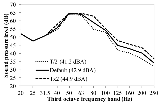
Figure 6: influence of reverberation time (T) on structure-borne noise levels in a small room
