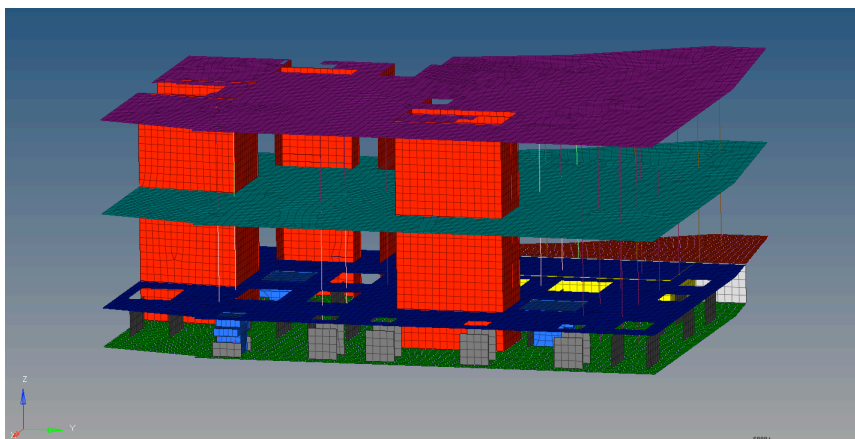
Figure 1: FE model of a science building
