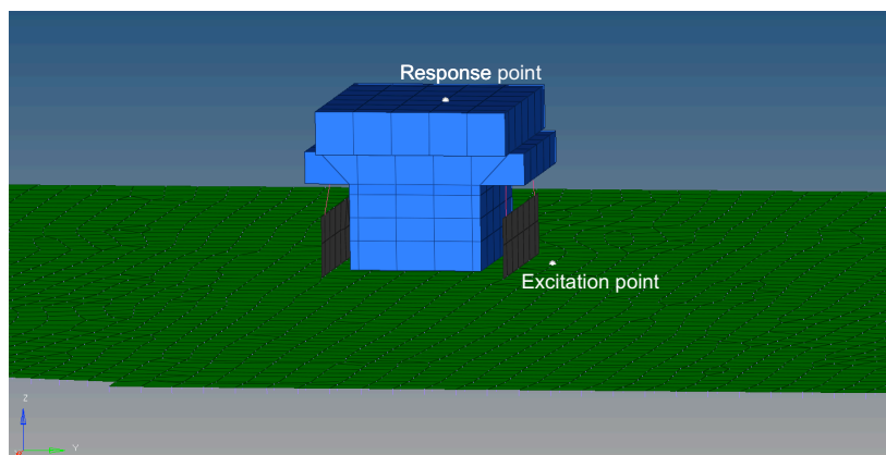
Figure 4: 50-ton concrete keel block supported by air springs mounted on support walls and foundation slab
