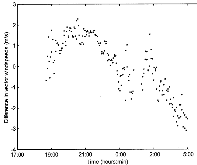
Figure 1: Difference between vector winds at height 2m at source and height 2m at 1km for 150s averages
