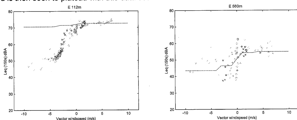
Figure 3: Correlating measured L_{Aeq}(150s) with vector wind speed for measurements over grass. Comparisons with CONCAWE (--)
