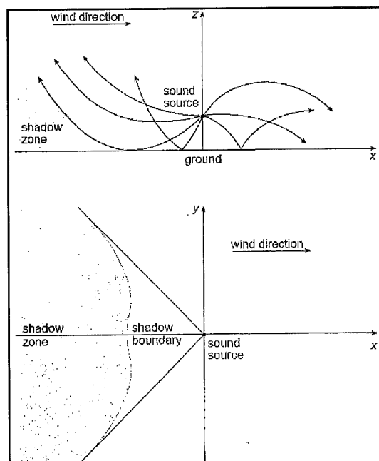
Figure 2: Sound wave refraction and shadow zone formation associated with a temperature inversion and a wind velocity gradient
