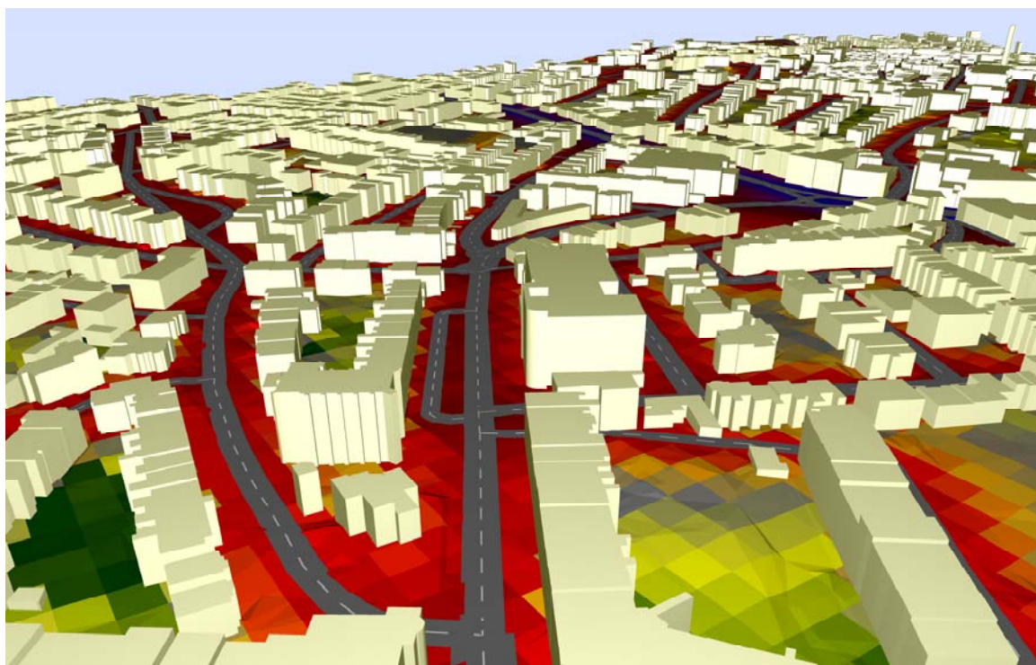
Figure 6: Three-Dimensional View of the Bristol Noise Map with Noise Contours
