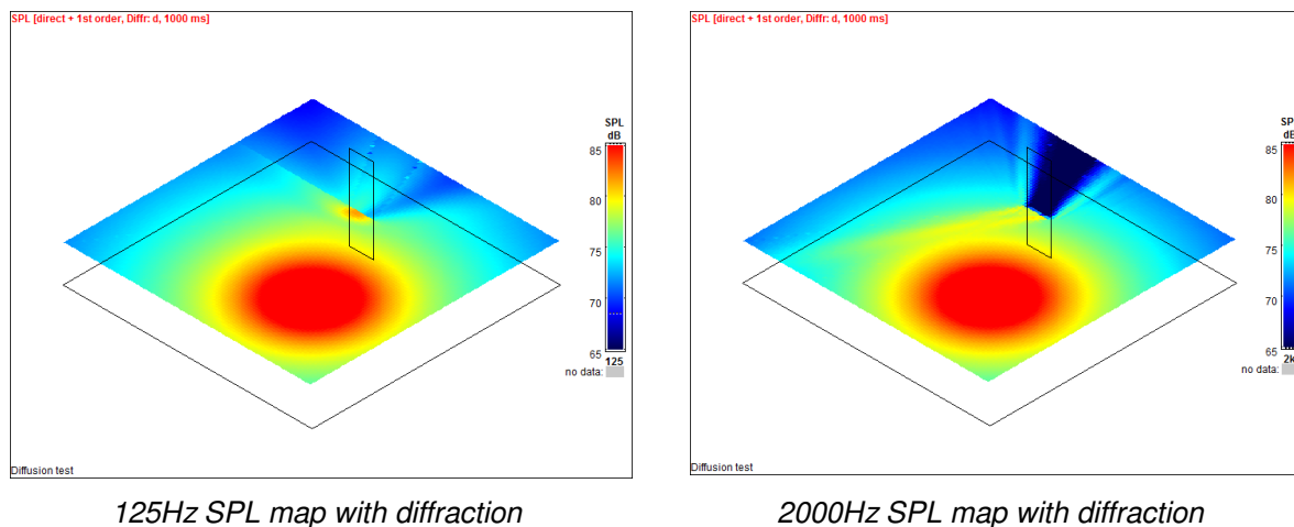
Figure 5 - Comparison of diffraction in SPL maps close to a free-standing plane
