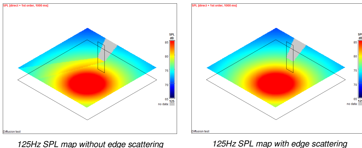
Figure 4 – Comparison of edge scattering in 125Hz SPL maps close to a free-standing plane
