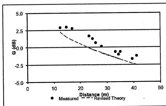
Figure 13 Measured Strength ( G ) compared to a Revised Theory prediction might explain the better than expected Intimacy. (1kHz octave)
