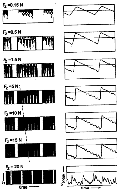
Figure 5: Friction maps and bridge-force waveforms as functions of bow force (from Pitteroff). White areas in the friction maps (left column) show sliding friction, which happens even during the "static interval" on the bridge side of the hair ribbon.
