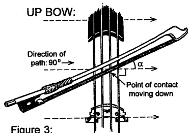
Figure 3: In certain situations, bowing with an angle to the string gives a better sound.
