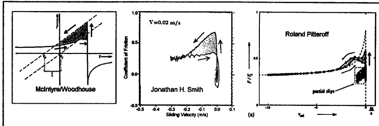
Figure 4: Three examples of frictional paths (see text).
