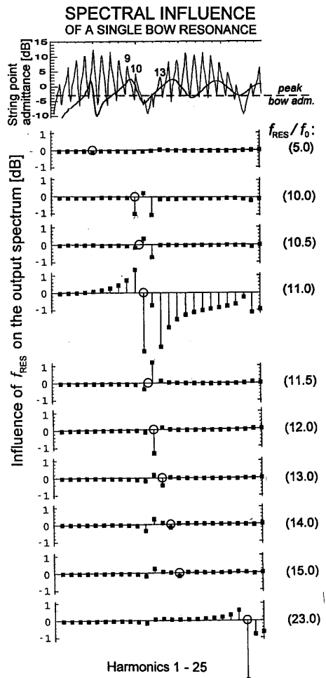
Figure 10 (right): Simulated influence of a bow resonance on the output bridge spectrum. The upper graph shows transversal (thin line) and torsional (bold line) point admittances for a string with characteristic wave resistances of 370 and 975 g/s, respectively. The fractional bowing point ( \beta ) is equal to 0.087 = 1/11.5 . The horizontal dashed line shows the peak level of the bow's admittance at its resonance frequency f_{RES} . Below, the difference between the output spectrum of a string bowed with a resonant and a nonresonant bow is shown for 10 different f_{RES} . The relative frequency f_{RES}/f_0 is marked with a circle in each plot. Notice that when f_{RES} exactly matches the frequency of a string harmonic, this harmonic will be lowered in the bridge output spectrum. All simulations were run with the same bow velocity and bow force. The durations of the resulting stick-slip intervals turned out to be identical in all simulations.
