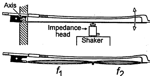
Figure 7: Examples of transversal "hair modes" on each side of the excitation point.
