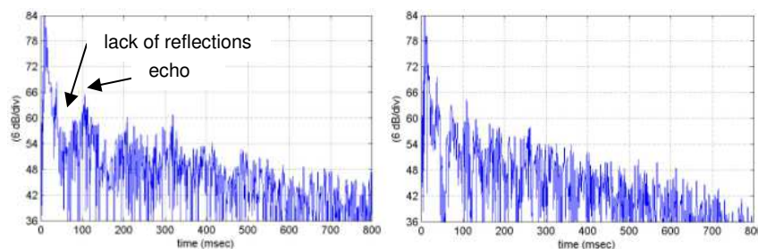
Figure 6. Typical difference in scale model impulse response of a 1m position on stage (hearing your own instrument) at Q2 (trumpets) without stage reflector 2012 (left) and with stage reflector 2015 (right), (scaled to) 1kHz.
