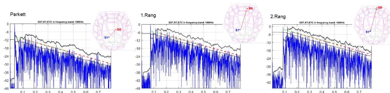
Figure 8. Three measured impulse responses in the final hall, unseated, 1kHz.
