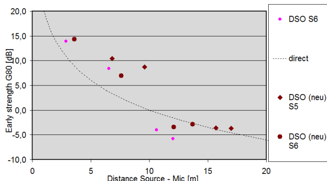
Figure 22. Measured Early Strength G_{80} before (violet) and after renovation (brown): sources in the pit and receivers on stage.
