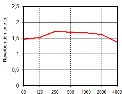
Figure 19. Measured RT with interrupted noise and pistol(63 Hz) in 2017. Concert situation
