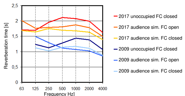
Figure 18. Measured RT with interrupted noise and pistol (63 Hz) in 2009 and 2017. Opera situation.
