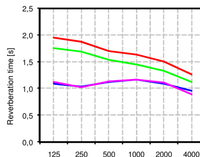
Figure 5. measured and calculated RT with audience (simulation). Violet: exiting measured FC closed, Blue: existing calculated, Red: new with FC closed, Green: new with FC open.
