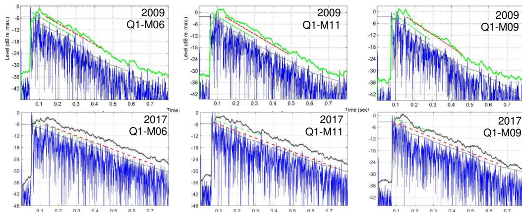
Figure 17. Some measured IR's from 2009 (top) and 2017 (bottom). Opera situation with closed FC and audience simulation.
