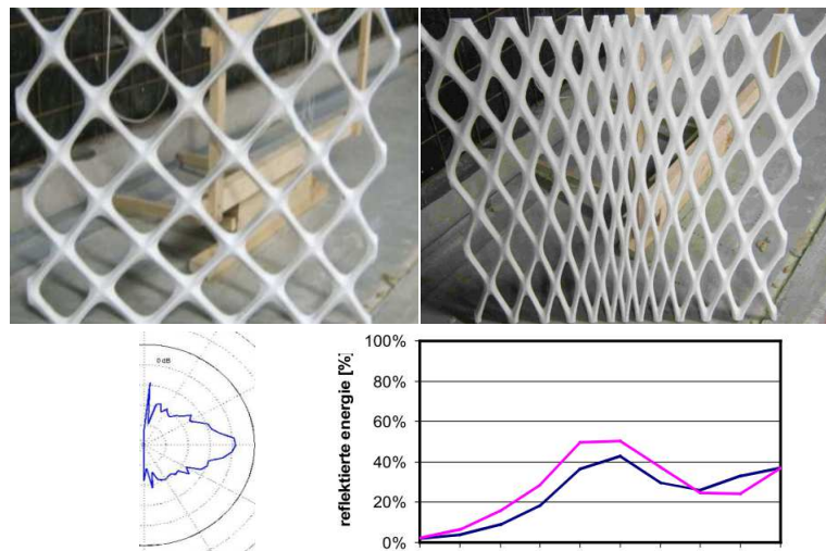
Figure 13. Measurements of the grid structure scale 1:2. Top: both samples, bottom left: directional reflection (6dB/div). Bottom right: total reflected energy [%], blue: left sample, violet: right sample.
