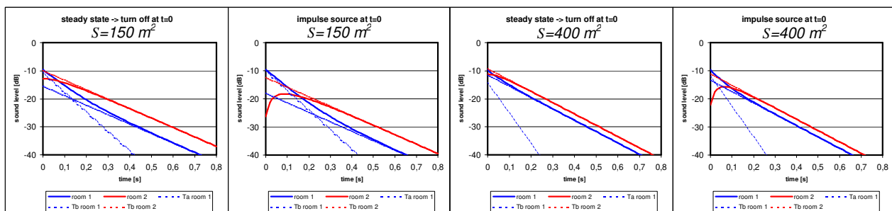
Figure 3. Diffuse field sound decay after switching off a steady state signal or after an impulse signal, room 1: 6500 m 3 , room 2: 3000 m 3 , coupling surface S : 150 m 2 (left) or 400 m 2 (right).
