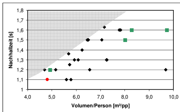
Figure 1. Measure reverberation times (1 kHz, occupied) related to the specific volume for 32 opera halls 2 . The green squares are opera halls that were judged to be very good 2 . Red: State opera Berlin.
