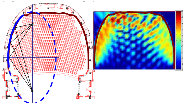
Figure 9. Floor plan of stalls (left) with the segment of an ellipse (blue) and sources and receiver points that result in focussing. Right: calculation 5 of the first reflection (125 Hz).
