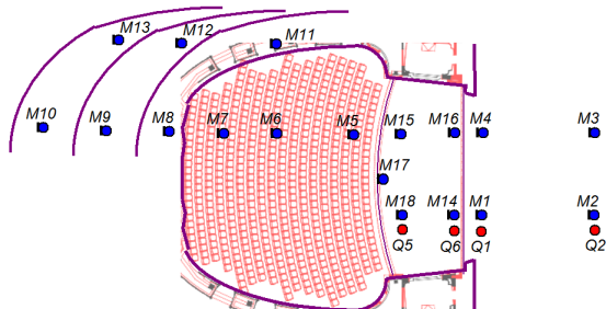
Figure 16. Sources (in red) and receivers (in blue). Balconies are schematic. Not shown: source position 7 in the pit (under Q1).
