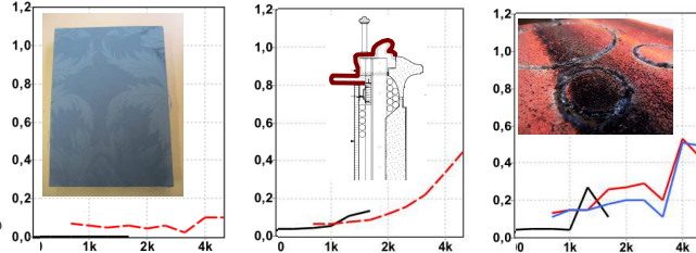
Figure 11. Measured sound absorption in the interferometer, after optimisation. Left: wall finishing (glued woven textile), middle: railings (glued velvet), right: wall above stage opening (glued velours).
