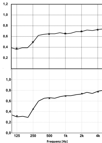
Figure 12. Sound absorption of 16 seats, measured in occupied situation. Top: existing seats, bottom: new seats.
