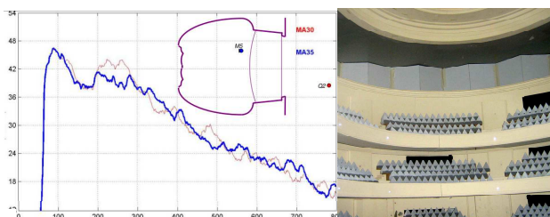
Figure 8. Measured and smoothed (20 ms) impulse response ETC from the stage to front of stalls. Left: red is with elliptical wall, blue is with folded walls.
