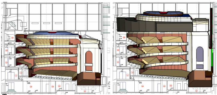
Figure 4. acoustic calculation model overlaying the longitudinal section of the hall. Left: existing before 2010, right: final design.
