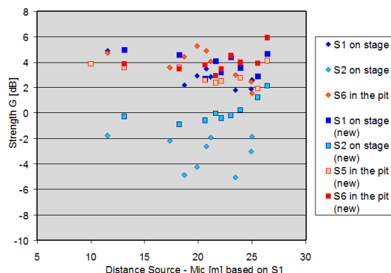
Figure 20. Measured strength G before (wybers) and after renovation (squares).
