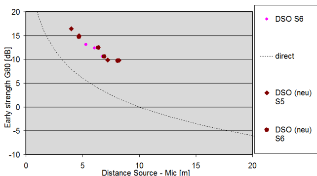
Figure 21. Measured Early Strength G_{80} before (violet) and after renovation (brown): sources and receivers in the pit
