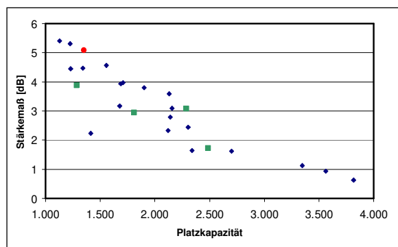
Figure 2. Strength G (1 kHz, occupied) related to the number of audience for 32 opera halls. The green squares are opera halls that were judged to be very good 2 . Red: State opera Berlin
