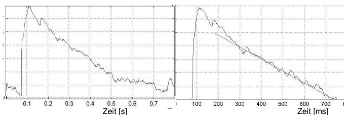
Figure 7. Measured and smoothed (20 ms) impulse response ETC from fore stage to middle of 3 d balcony of existing hall (before 2010). Left: 1:1, right: 1:10. 6 dB/div.
