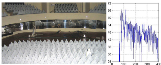
Figure 10. Left: scale model with curved mirrors on the walls, right: measured ETC in the focal point.
