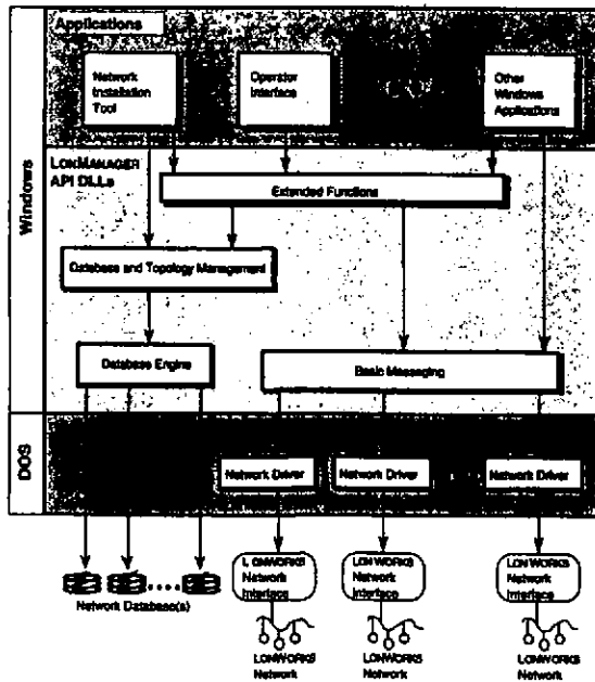
Figure 2 LONWORKS API Overview
