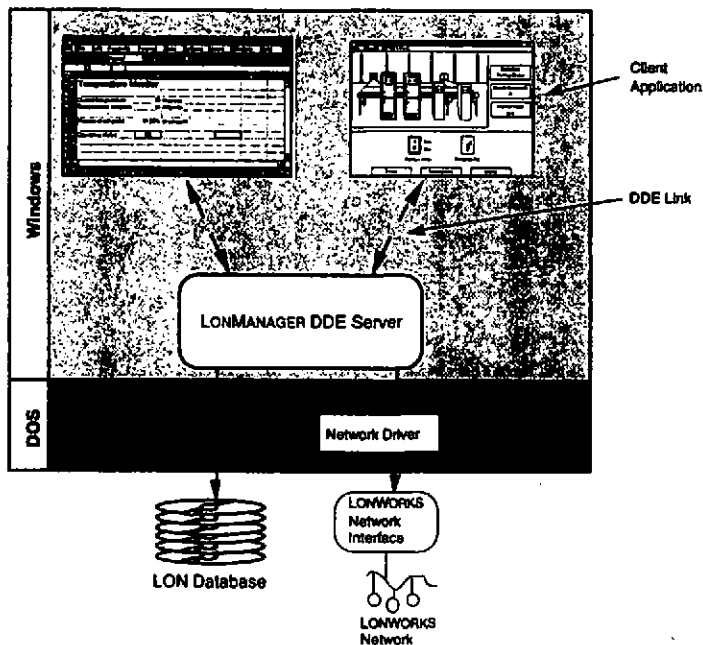
Figure 1 LONWORKS DDE Server Overview
