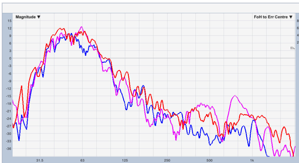
Figure 8: Smart RTA measurements at the point of immission. The transfer function of three error microphone positions (shown in figure 7) are plotted. The data is smoothed over 1/12 octave.
