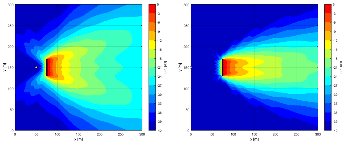
Figure 3: Simulations of SPL coverage patterns for array delays corresponding to a virtual point source (shown as white point). The left image shows a wide opening angle which results from a virtual point source at a distance of 25 m to the array. The image to the right depicts a narrower opening angle due to a longer distance of 75 m. The frequency used in this simulation is 63 Hz, the spacing between the speakers is 2 m and a tukey tapering function was utilized (this will be explained further down).
