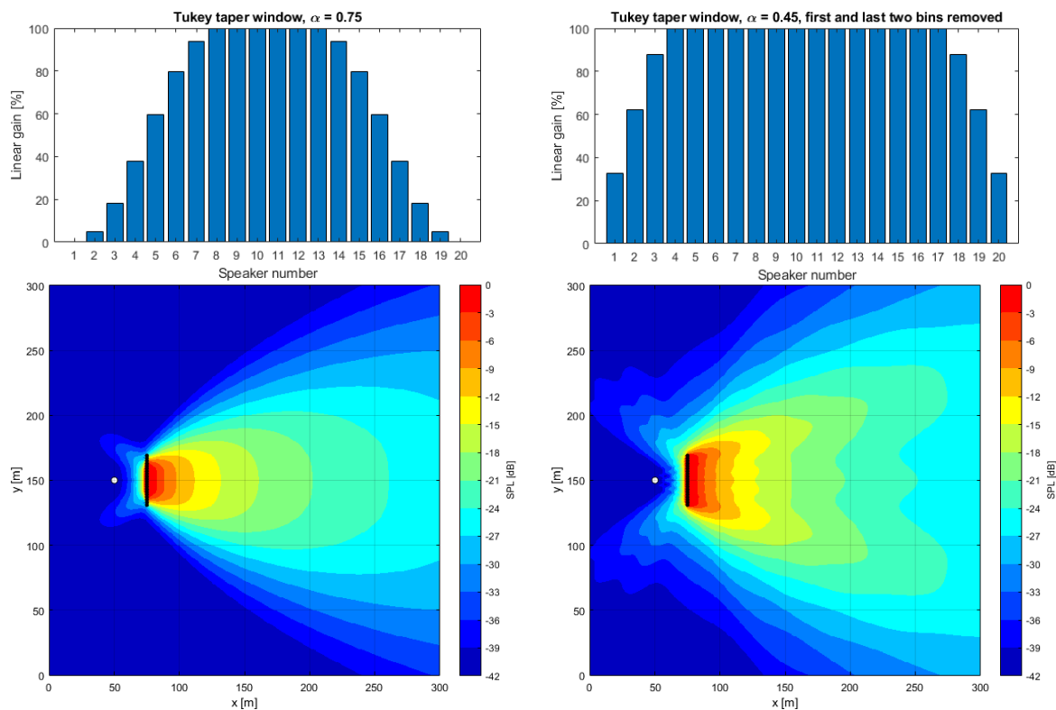
Figure 4: Simulation results using a tukey window tapering function. The simulation shows a cardioid sub array of 20 speakers with 2 m spacing at 63 Hz. The virtual point source is placed 25 m behind the array. On the left side the linear gains of a tukey window function with parameter 3 \alpha = 0.75 are shown. This produces a very homogenous field in front of the array. On the downside these settings result in an overall loss of -4.5 dB, which is not considered to be economical. The images on the right side show a more economical setting, using a tukey window with parameter \alpha = 0.45 . The window shown here was calculated for 24 instead of 20 speakers, but the 4 speakers with lowest amplitudes were simply neglected. This leads to an overall loss of only -1.1 dB, while still delivering acceptable results.
