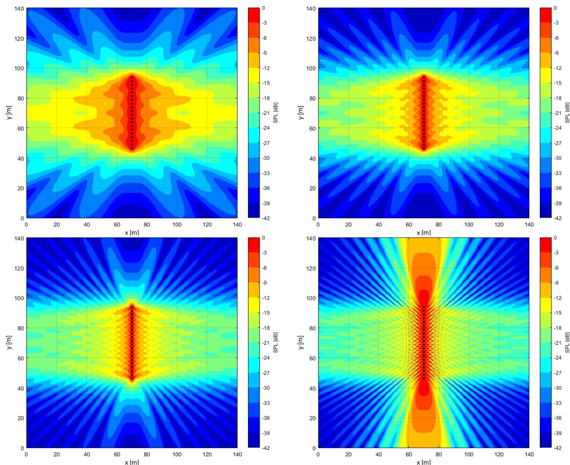
Figure 2: Simulation results for an element spacing of 2.5m. From left to right and top to bottom the images show SPL coverage patterns for following frequencies: 34 Hz ( \lambda = 1/4 spacing), 69 Hz ( \lambda = 2/4 spacing), 103 Hz ( \lambda = 3/4 spacing) and 137 Hz ( \lambda = 4/4 spacing).
