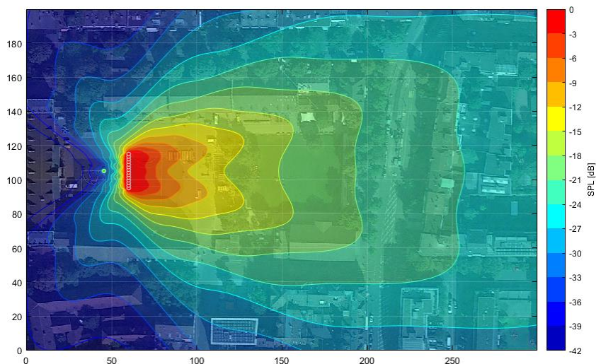
Figure 6: Simulation results of the sound pressure level produced by the main array (red dots) at a live concert. The virtual point source is shown as a green dot. The array is parametrized in a way to produce a homogeneous sound pressure distribution.
