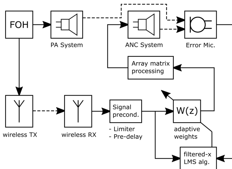
Figure 5: Simplified diagram of the SISO (Single-In-Single-Out) filtered-x LMS algorithm and its implementation in the sound reinforcement system.
