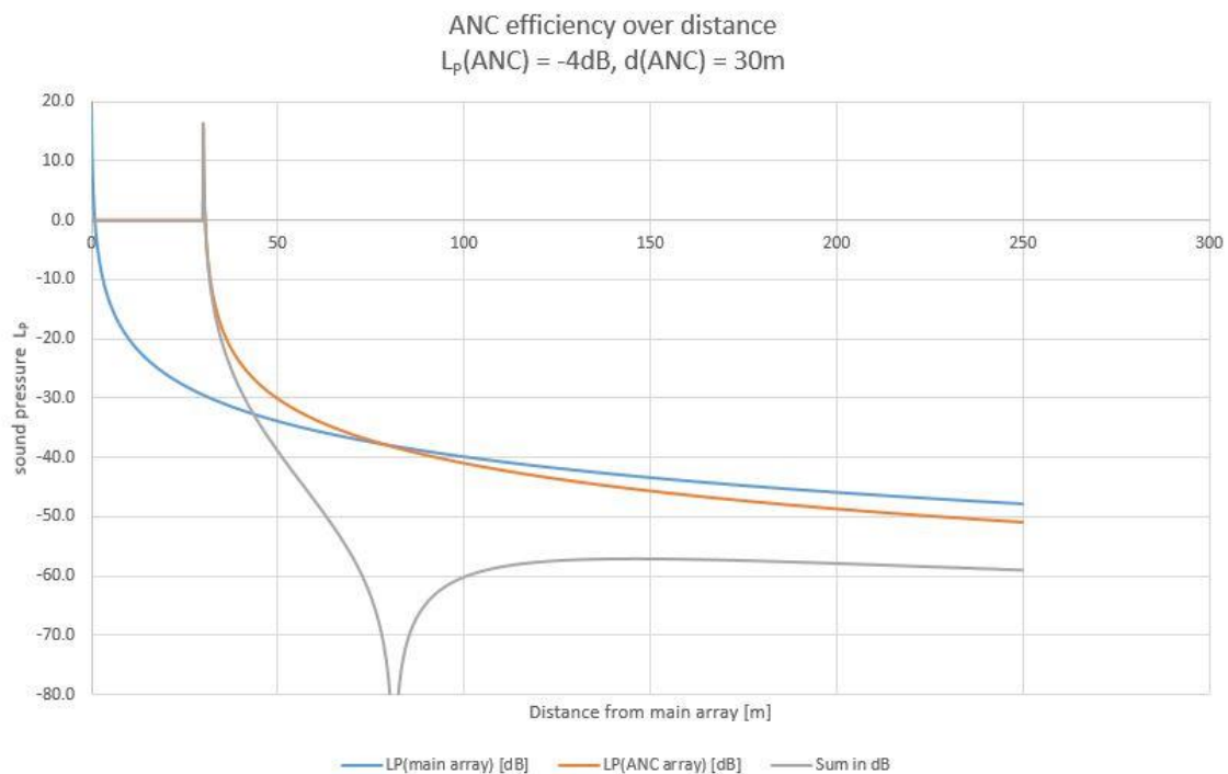
Figure 5: Simulation of the ANC efficiency over large distances. The sound pressures of the main array, the ANC array and their resulting sum are plotted against distance. The ANC is placed in a distance of 30 m from the main array with a sound pressure level 4 dB lower compared to the main array.
