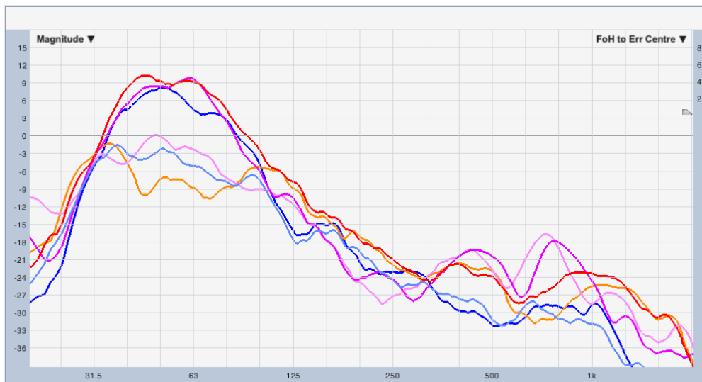
Figure 9: Efficiency of the LMS-based ANC algorithm. The bright lines show measurements while the ANC system is turned on, compared to the dark lines where the ANC System is turned off. A SPL reduction up to 18 dB is achieved around 50 Hz. The data is smoothed over 1/3 oct. The red (ANC off) and the orange (ANC on) curves belong to the central measurement position in figure 7. The other four curves belong to the lateral microphone positions.
