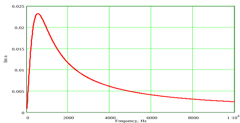
Figure 2. Imaginary part of the refractive coefficient n(\omega) for a medium with relaxation defined by Equation (6).
