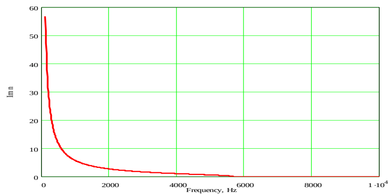
Figure 5. Imaginary part of the refractive coefficient n(\omega) for the first mode ( m = 1 ) of a waveguide with rigid walls defined by Equation (7).
