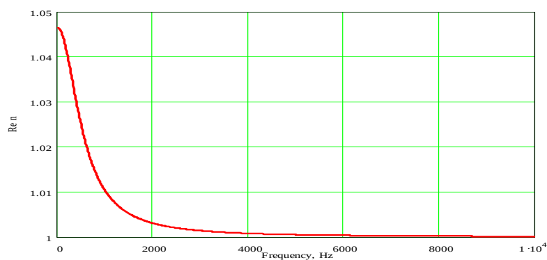
Figure 1. Real part of the refractive coefficient n(\omega) for a medium with relaxation defined by Equation (6).
