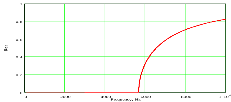
Figure 4. Real part of the refractive coefficient n(\omega) for the first mode ( m = 1 ) of a waveguide with rigid walls defined by Equation (7).
