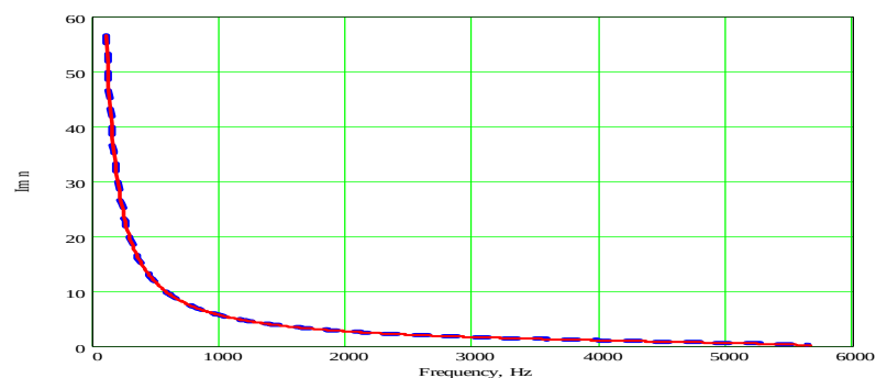
Figure 6. Imaginary part of the refractive coefficient n(\omega) for the first mode ( m = 1 ) of a waveguide with rigid walls defined by Equation (7) (solid curve) and calculated using Kramers-Kronig relation (9) (dashed curve).
