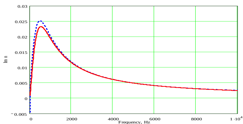
Figure 3. Imaginary part of the refractive coefficient n(\omega) for a medium with relaxation defined by Equation (6) (solid curve) and calculated using Kramers-Kronig relation (4) (dashed curve).
