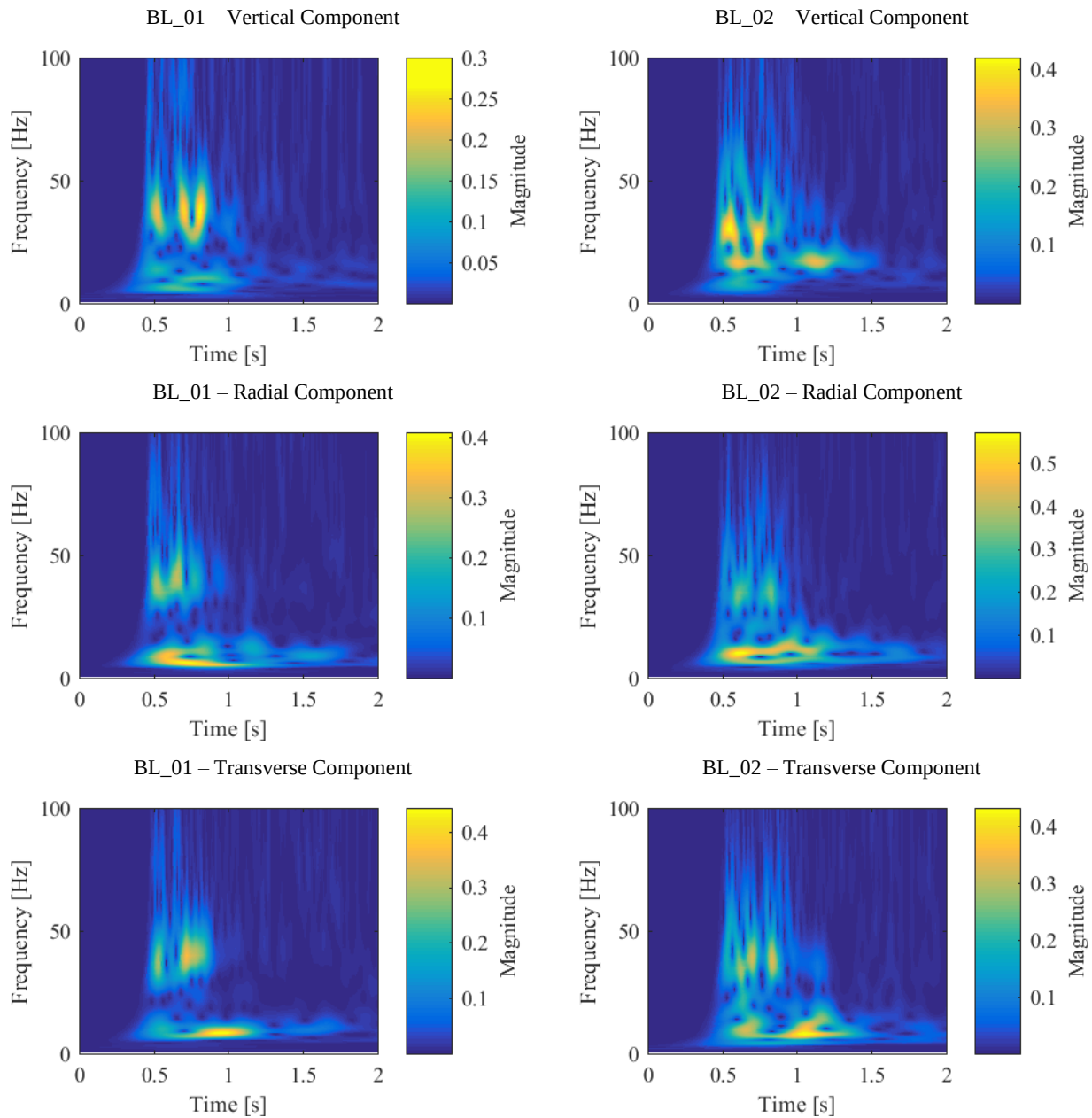
Figure 8: Time-frequency analysis using the Continuous Wavelet Transform ( N_{oct} = 10 , N_{voi} = 10 ) of the vertical, radial, and transverse components of the two blast-induced ground vibration records.
