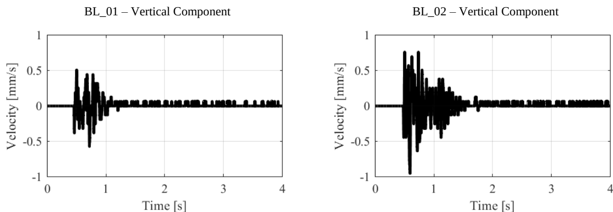
Figure 5: Sample time histories of the blast-induced ground vibrations analysed in this paper.
