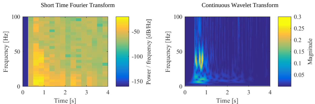
Figure 7: Comparison of the time-frequency analysis of the vertical component of the ground vibration record BL_01 using (a) the Short Time Fourier Transform ( \delta t = 0.25 \text{ s} / \Delta f = 4.00 \text{ Hz} ), and (b) the Continuous Wavelet Transform ( N_{oct} = 10, N_{voi} = 10 ).
