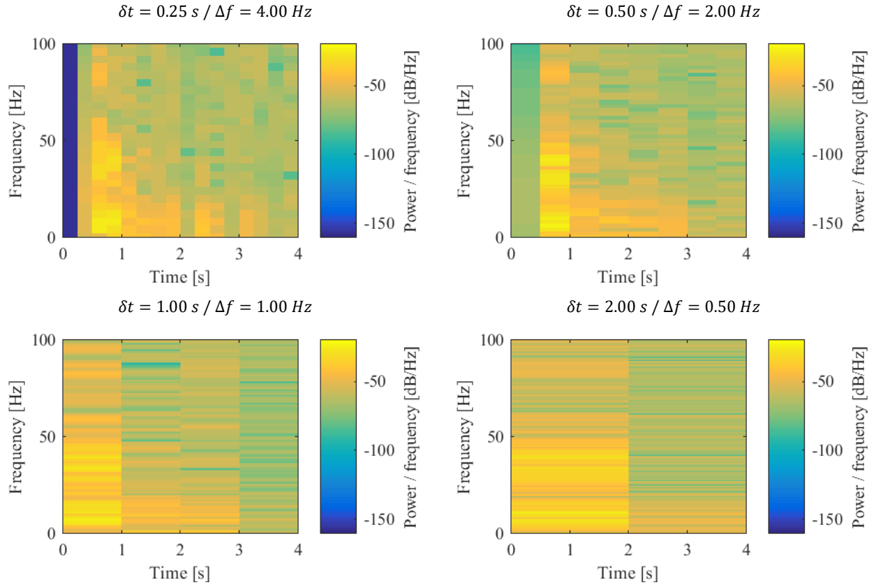
Figure 6: Comparison of the influence of varying the sub-record length ( \delta t ) of the Short Time Fourier Transform on the time-frequency analysis of the vertical vibration component from record BL_01.
