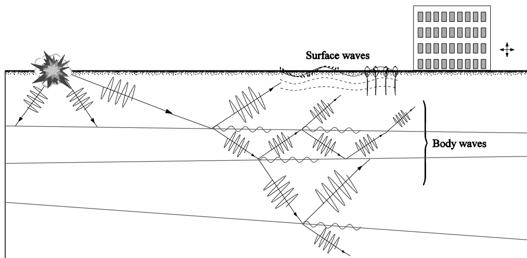
Figure 1: An illustration of the propagation of body and surface waves generated by an explosive blast.
