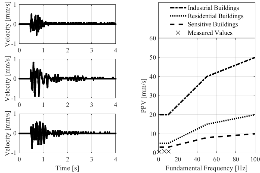
Figure 2: Typical example of blast-induced ground vibration analysis, with the measured vertical, radial, and transverse time histories, and the results presented on the DIN 4150-3 Z-Curve (right).
