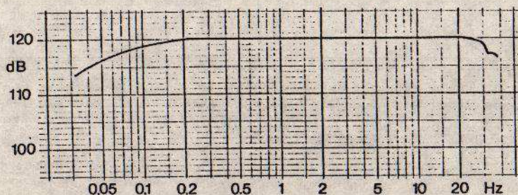
Figure 2. Measurement of the sound pressure level in the test chamber with 1 V at the input of the frequency and gain correcting circuit.
