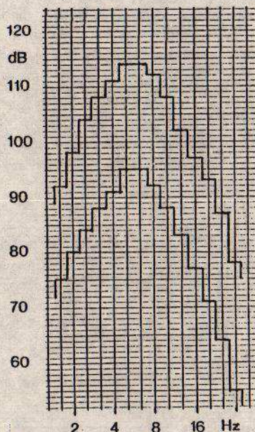
Figure 5. A 1/3 octave analysis of the two infrasound noise spectra used in the experiments.
