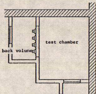
Figure 1. The infrasound laboratory.
