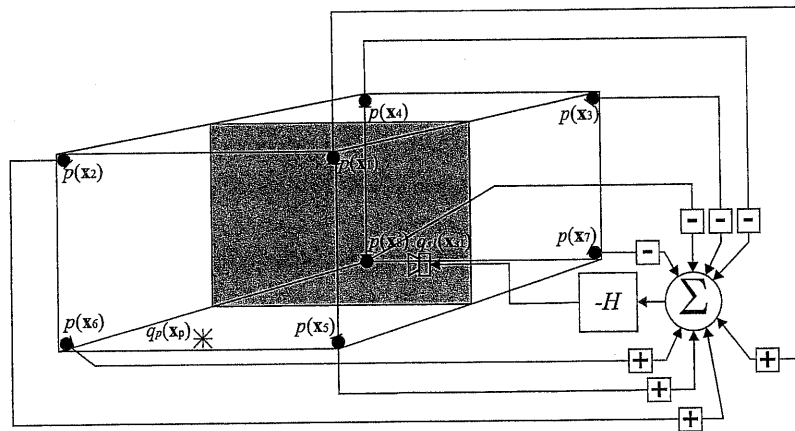
Figure 2: Modal feedback control system.
