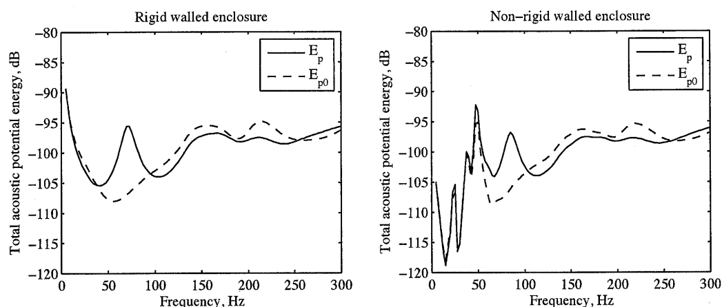
Figure 4: Total acoustic potential energy in the rigid and non-rigid enclosures when driven by a primary source alone (solid lines) and when the modal feedback control strategy using a single secondary source positioned as shown in Figure 2 has been employed with a maximum error signal enhancement of 6 dB (dashed lines).
