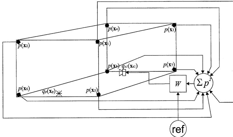
Figure 1: Global feedforward control strategy.
