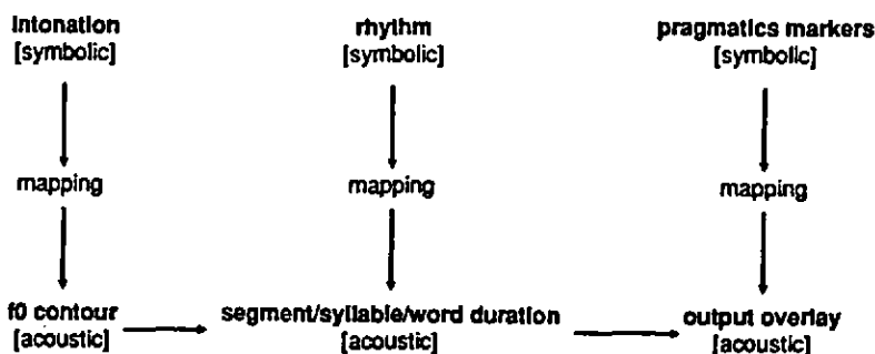
Fig.2 The relationship between symbolic and acoustic levels in the model.
