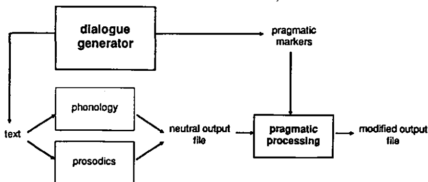
Fig.1 The overall model for generating a pragmatically modified output file.
