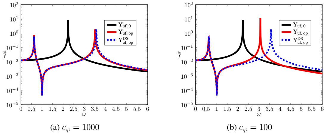
Figure 3: FRF between impact point h in y-direction and sensor k in y-direction (cf. figure 2b). Comparison of idle FRF Y_{uf,0} , reference solution Y_{uf,op} , and dynamic substructuring result Y_{uf,op}^{DS} , obtained with the violated kinematic assumption.
