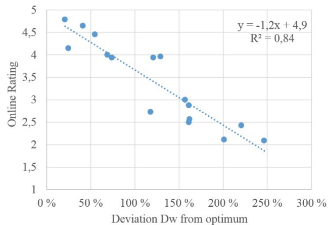
Figure 5: Regression analysis of the halls in group R16
