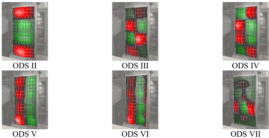
Figure 5: Operational Deflection Shapes.
