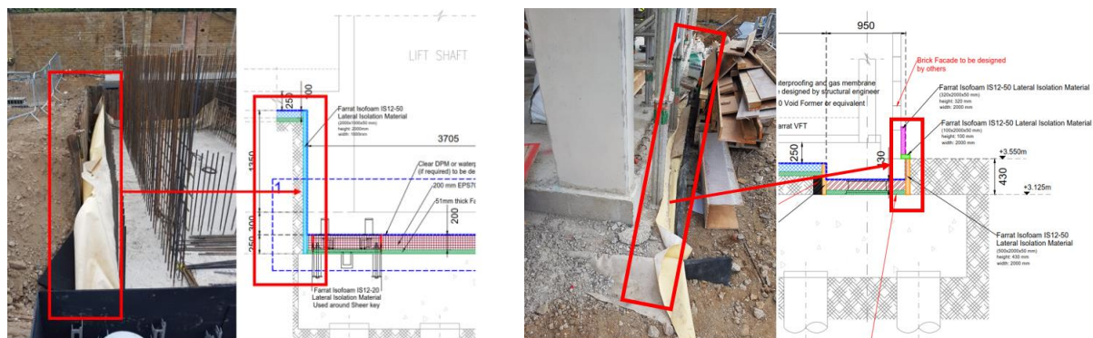
Figure 2: Typical examples of the challenges of constructing robustly isolated details
