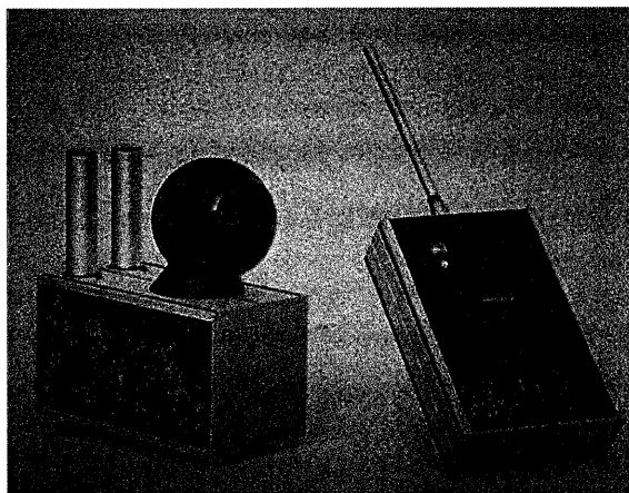
Figure 2. First implementation of RASTI in hardware (1980).
