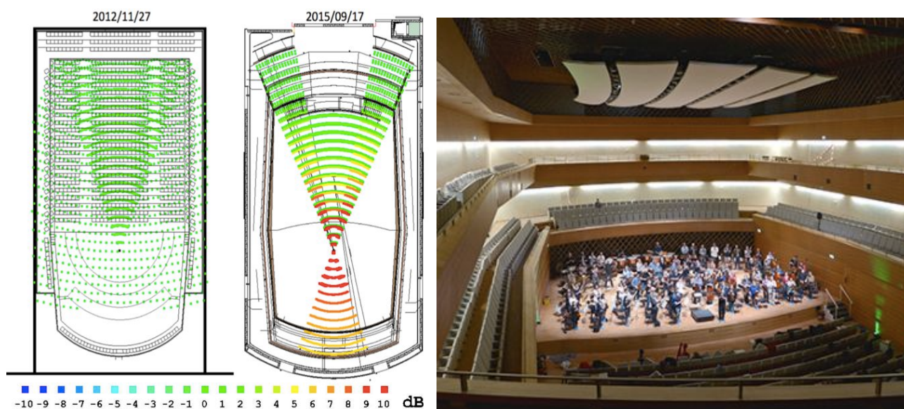
Figure 3: From left to right, evolution of the plan shape of Musikforum Bochum between competition phase (2012) and executed design (2015) with indication of the theoretical 2D focusing amplitude; the first test concert (2016) confirmed that any issues of focusing had been solved in 3D reality.
