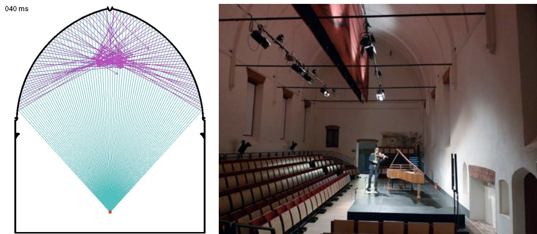
Figure 7: variable absorption located in the focal point of the vault of Kraakhuis, Ghent.
