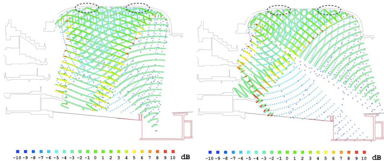
Figure 1: Long-section showing the focusing effect of the dome of La Monnaie opera house, for a source in the orchestra pit (left image) and on stage (right image). The parameter plotted is \Delta L_{\text{curv}} . The parts of the dome creating the strongest focusing in the audience are indicated by dashed ovals.
