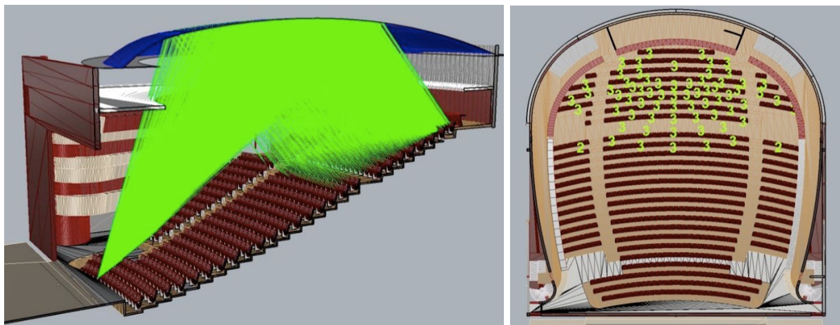
Figure 4: 3D raytrace of the proposed dome of the new Comédie of Clermont-Ferrand for a source near the stage edge, with indication of the focusing amplitude (in dB) in the rear half of the parterre.
