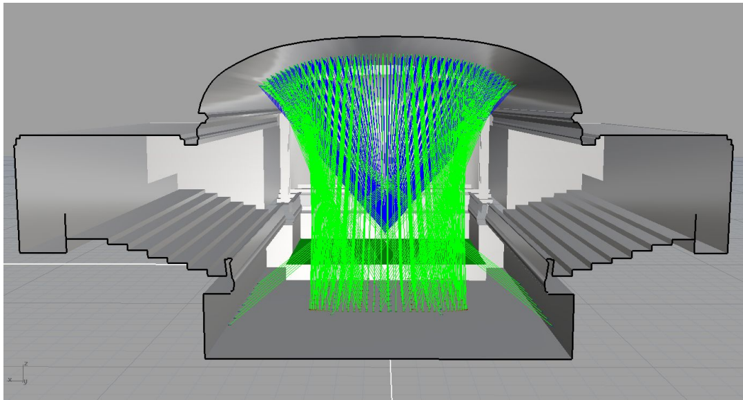
Figure 2: 3D raytrace of the concave ceiling of Kulturcasino, Bern (cross-section view), showing that a large portion of the parterre width is covered by mild focusing from the ceiling.
