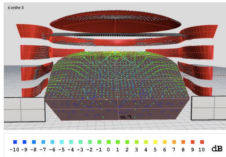
Figure 5: combined focusing study of the proposed bands and dome of the Comédie, showing the reflection coverage for reflections up to 3 rd order, for a source 3m behind the stage edge.
