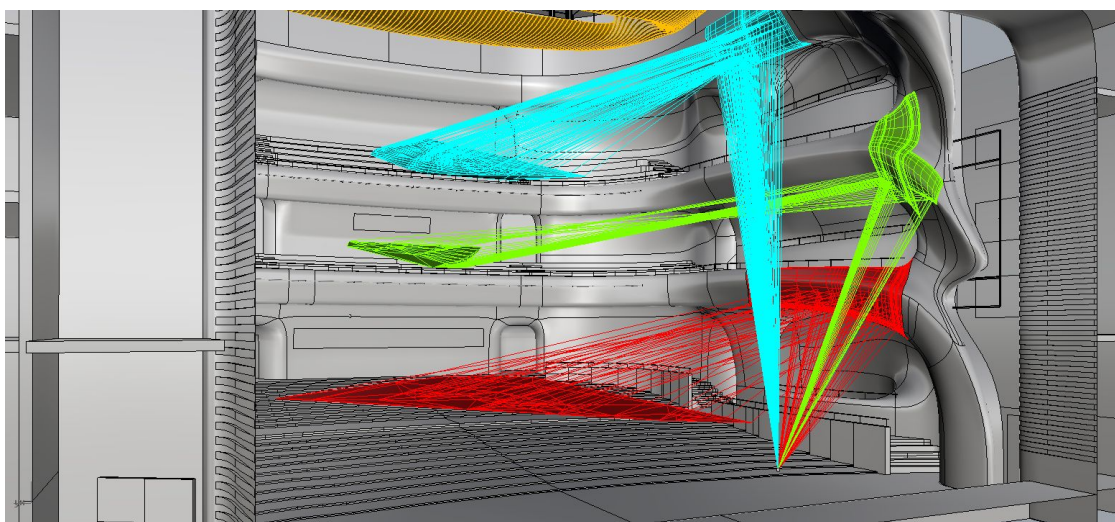
Figure 6: excerpt of 3D raytracing study in Rhino/Grasshopper of the acoustic shaping of the freeform walls of the Fuzhou Opera House.
