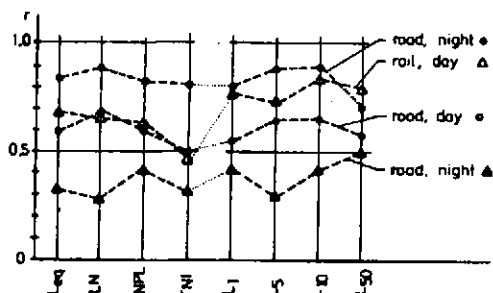
Fig. 2 Correlations (r) between acoustic indices and overall disturbance reactions for day, night and rail, road
